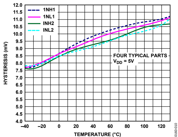
Figure 10. Hysteresis vs. Temperature for Four Typical Parts
