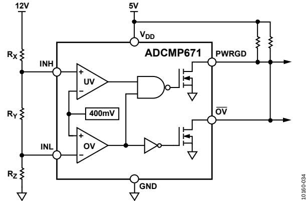
Figure 34. Undervoltage/Overvoltage Monitoring Configuration
