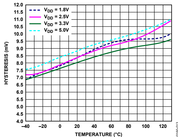
Figure 13. Hysteresis vs. Temperature for Various V_{DD} Voltages
