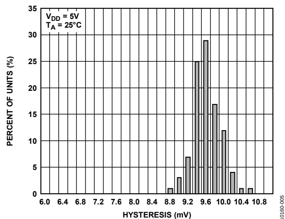
Figure 5. Distribution of Hysteresis
