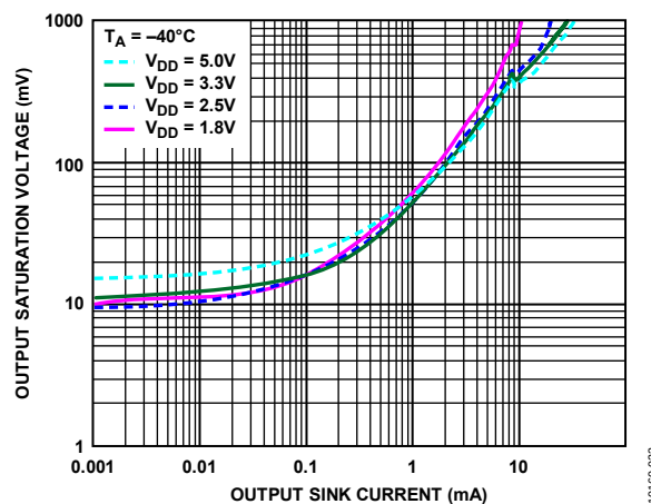
Figure 25. Output Saturation Voltage vs. Output Sink Current for T_A = -40^\circ\text{C}
