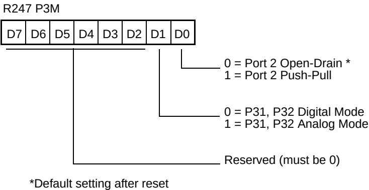
Figure 21. Port 3 Mode Register—F7H: Write Only
