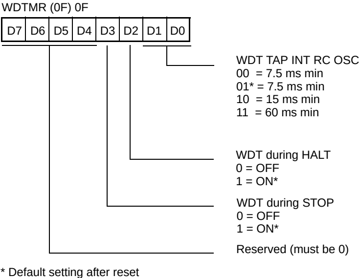
Figure 18. Watch-Dog Timer Register—(0F) 0FH: Write Only
