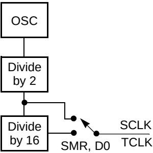
Figure 47. SCLK Circuit
