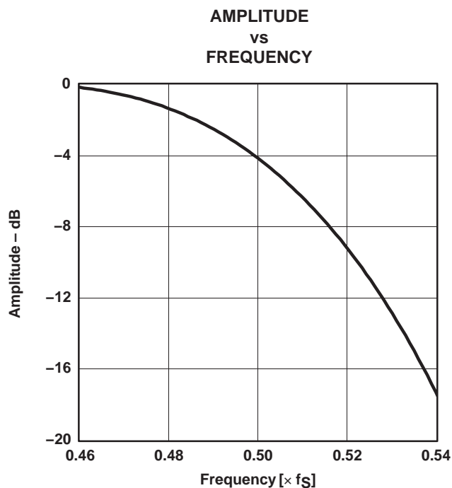
Figure 19. Transition-Band Response
