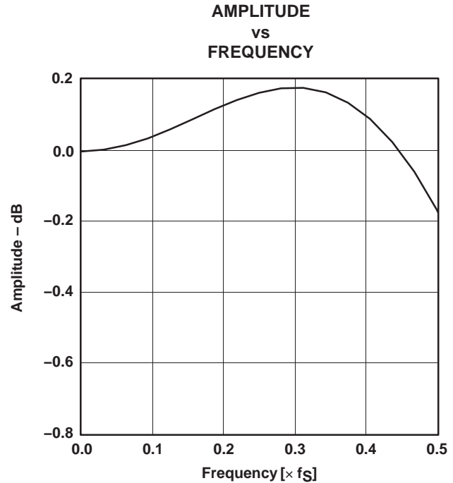
Figure 28. Pass-Band Characteristic
