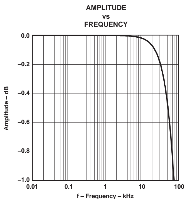
Figure 23. Pass-Band Characteristic
