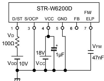
Measurement Circuit 10
