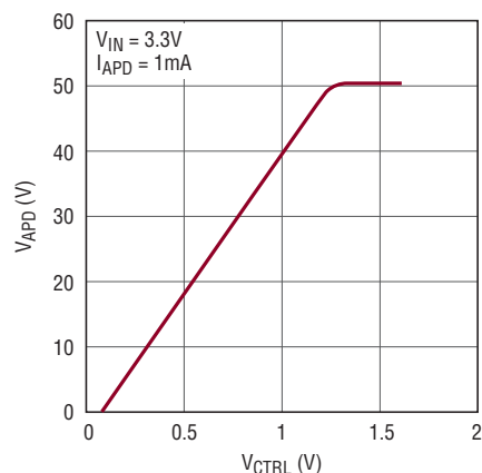
APD Voltage Adjustment with CTRL
