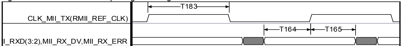
Figure 14-18. RMII Interface Input Signal Timing
