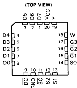
SN54HC354 . . . FK PACKAGE
