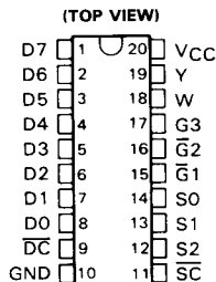
SN54HC354 . . . J PACKAGE SN74HC354 . . . DW OR N PACKAGE
