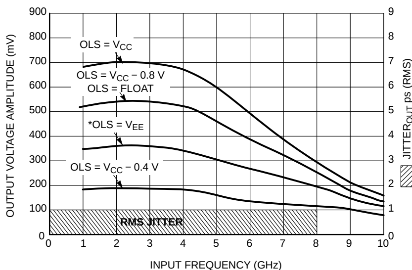
Figure 8. Output Voltage Amplitude ( V_{OUTPP} ) / RMS Jitter vs. Input Frequency ( f_{in} ) for 2:1 MUX Mode ( V_{CC} - V_{EE} = 3.3 V @ 25°C; Repetitive 1010 Input Data Pattern)
