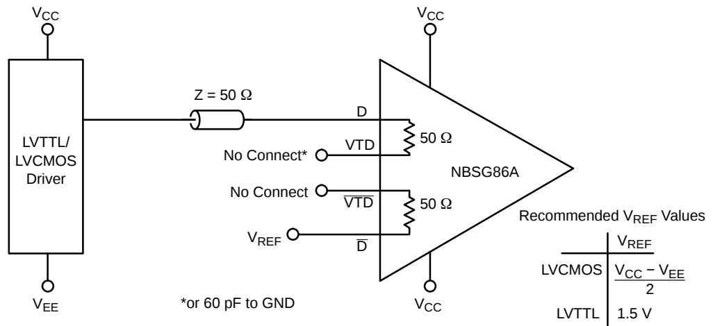
Figure 21. LVCMOS/LVTTL Interface
