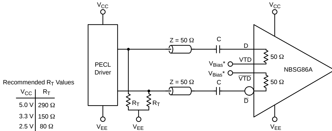
Figure 19. PECL Interface
