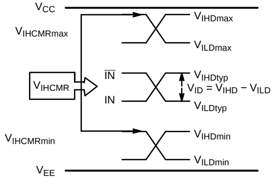
Figure 15. V_{IHCMR} Diagram
