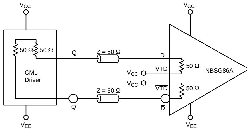
Figure 18. CML Interface
