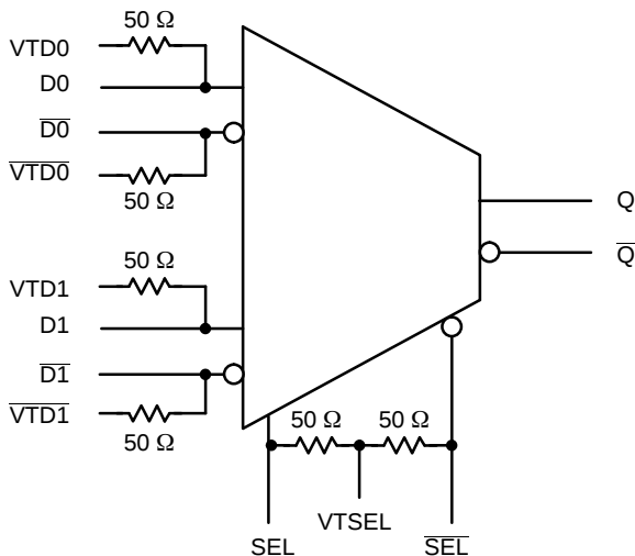
Figure 6. Configuration for 2:1 MUX Function
