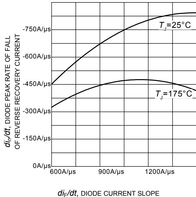
Figure 26. Typical diode peak rate of fall of reverse recovery current as a function of diode current slope ( V_R = 400\text{V} , I_F = 20\text{A} , Dynamic test circuit in Figure E)
