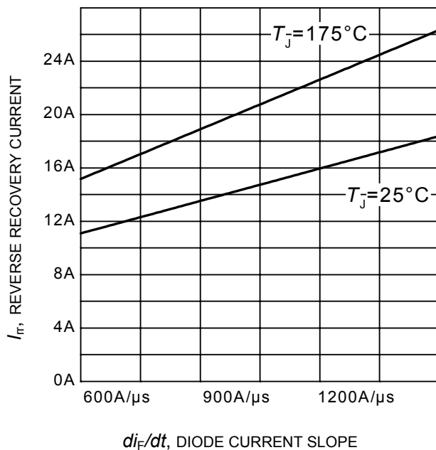
Figure 25. Typical reverse recovery current as a function of diode current slope ( V_R = 400\text{V} , I_F = 20\text{A} , Dynamic test circuit in Figure E)
