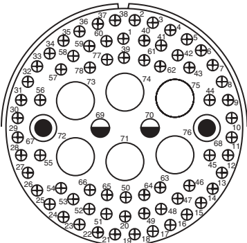
Insert Arrangement Service Rating Number of Contacts Contact Size 48-55 A 68 2 2 6 16 12 8 4
