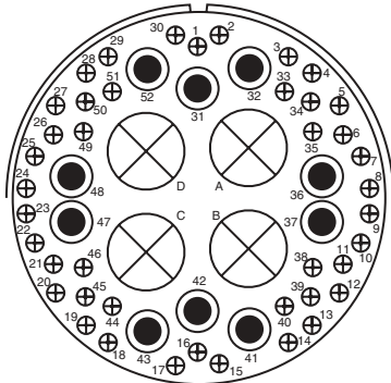
Insert Arrangement Service Rating Number of Contacts Contact Size 48-57 A 42 10 4 16 8 0
