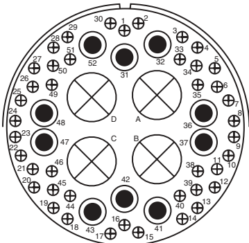
Insert Arrangement Service Rating Number of Contacts Contact Size 48-54 A 42 10 4 16 8 0 (Coax) RG-59/U
