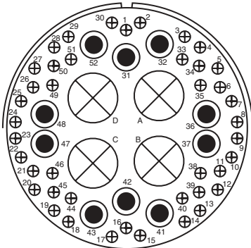
Insert Arrangement Service Rating Number of Contacts Contact Size 48-60 A 42 10 4 16 8 0 (Coax) RG-214/U
