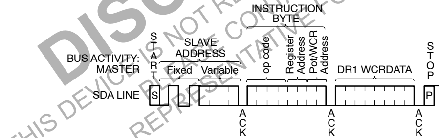
Figure 7. Write Timing
