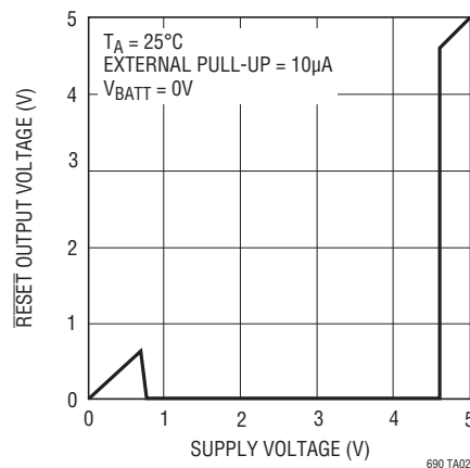
\overline{\text{RESET}} Output Voltage vs Supply Voltage
