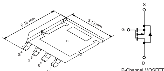
PowerPAK® SO-8L Single
