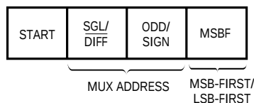
LTC1091 DATA INPUT ( D_{IN} ) WORD:
