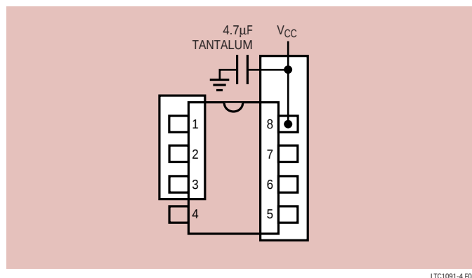
Figure 4. Example Ground Plane for the LTC1091
