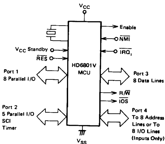
Figure 17 HD6801V MCU Expanded Non-Multiplexed Mode
