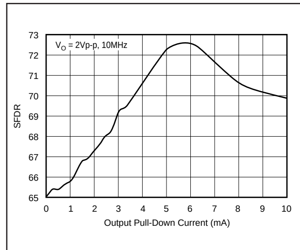
FIGURE 4. SFDR vs I_B .
