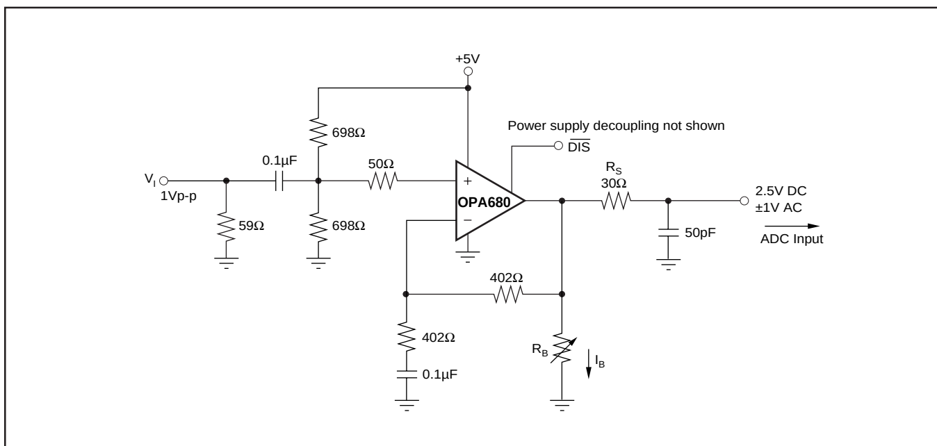
FIGURE 3. Single-Supply ADC Input Driver.
