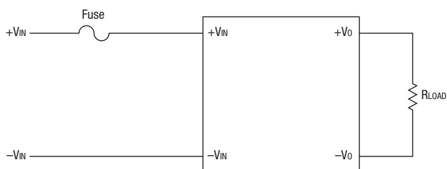
Figure 2. Input Fusing
