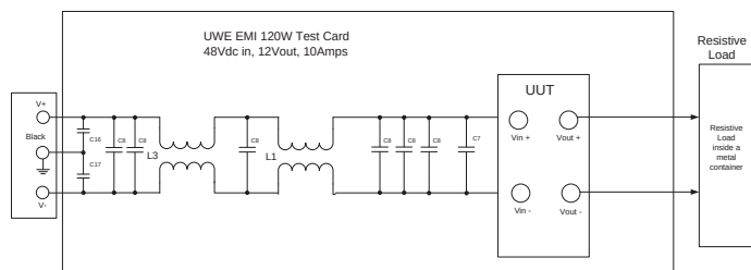
Figure 10. Conducted Emissions Test Circuit
