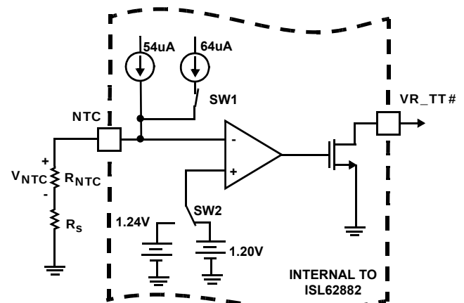
FIGURE 26. CIRCUITRY ASSOCIATED WITH THE THERMAL THROTTLING FEATURE OF THE ISL62882
