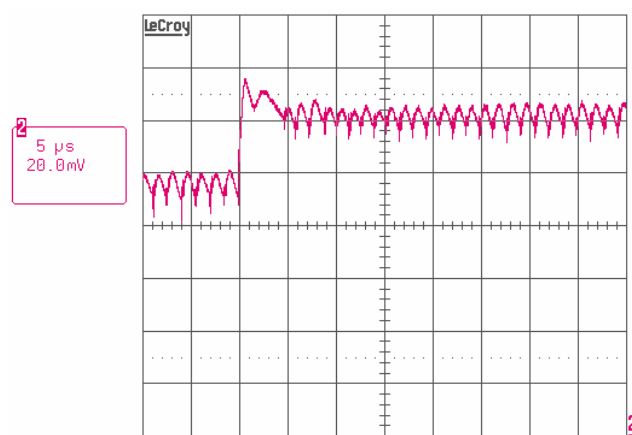
FIGURE 45. 2-PHASE MODE LOAD INSERTION RESPONSE WITH OVERSHOOT REDUCTION FUNCTION DISABLED, 3-PHASE CONFIGURATION, PSI# = 0, DPRSLPVR=0, V_{IN} = 12V , VID = 0.875V, I_O = 4A/17A , di/dt = "FASTEST"
