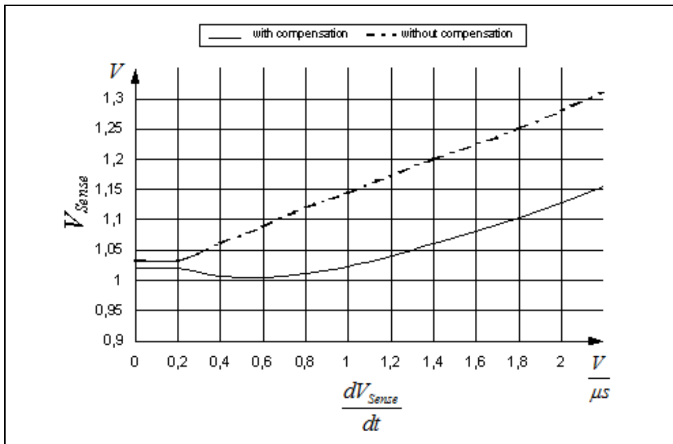
Figure 21 Overcurrent Shutdown
