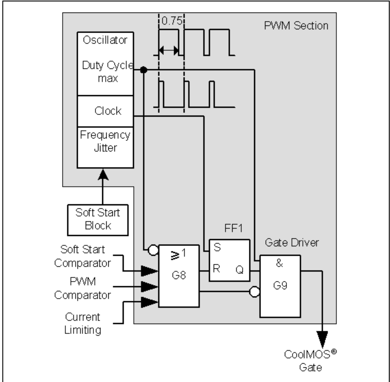
Figure 15 PWM Section Block
