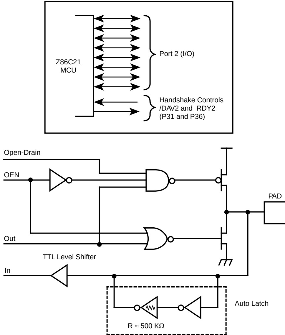
Figure 7. Port 2 Configuration
