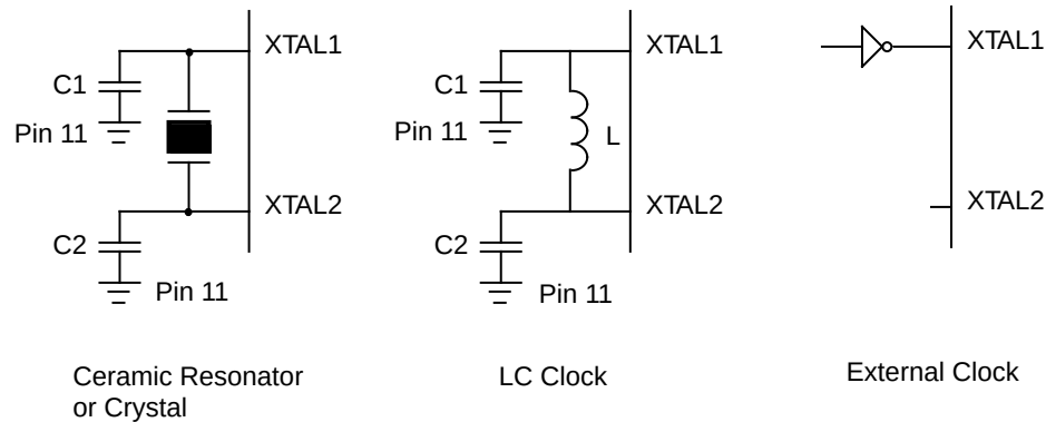
Figure 17. Oscillator Configuration
