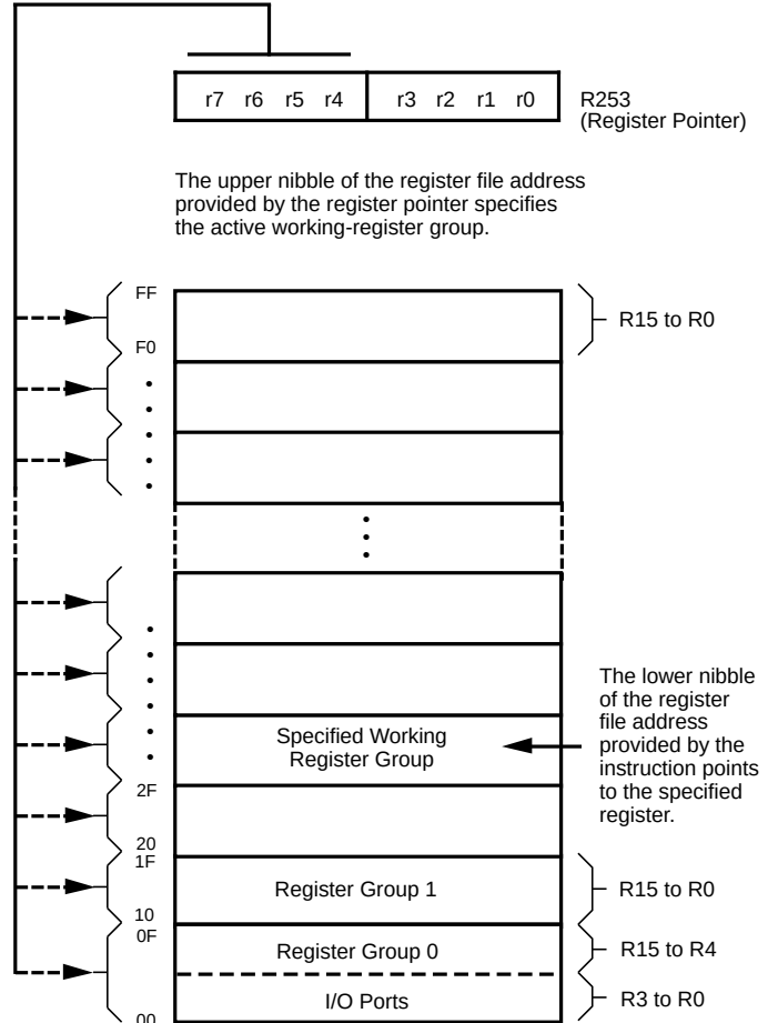
Figure 13. Register Pointer
