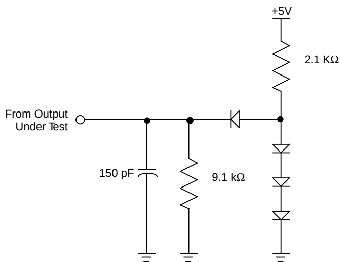
Figure 18. Test Load Diagram
