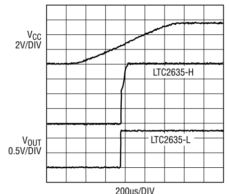
Power-On Reset to Mid-Scale
