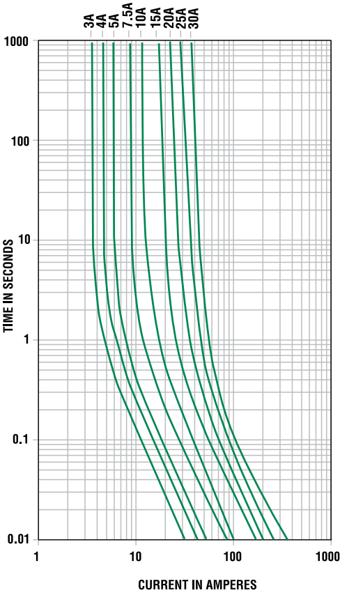
Time-Current Characteristic Curves
