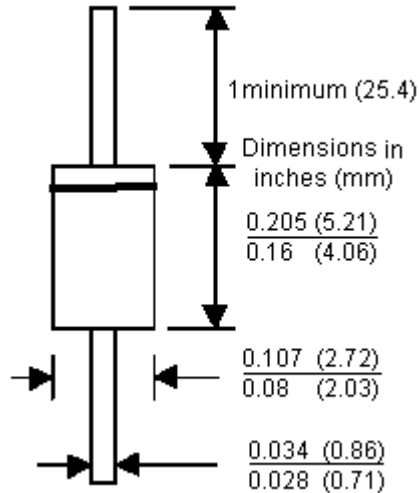
DO-41
