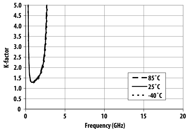
Figure 16. Over Temperature K-factor vs Frequency
