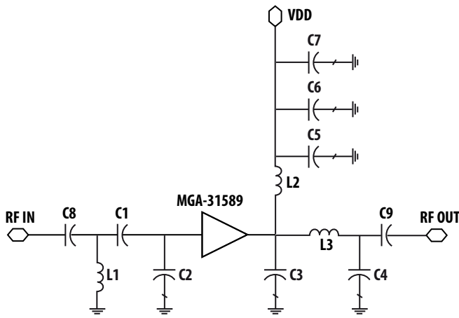
Figure 27. Circuit diagram
