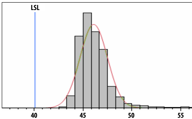
Figure 6. OIP3 at 900 MHz, Vdd = 5 V, LSL = 40.0 dBm, Nominal = 45.3 dBm
