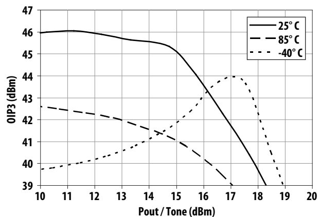
Figure 14. Over Temperature OIP3 at 700 MHz vs Pout
