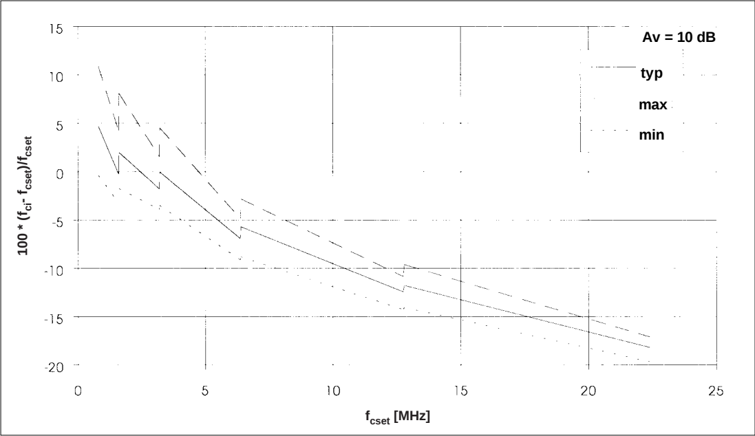
Figure 5: Measured cutoff frequency accuracy vs. settings ( V_{EE} = -5.00 V / T_a = 25^\circ\text{C} )
