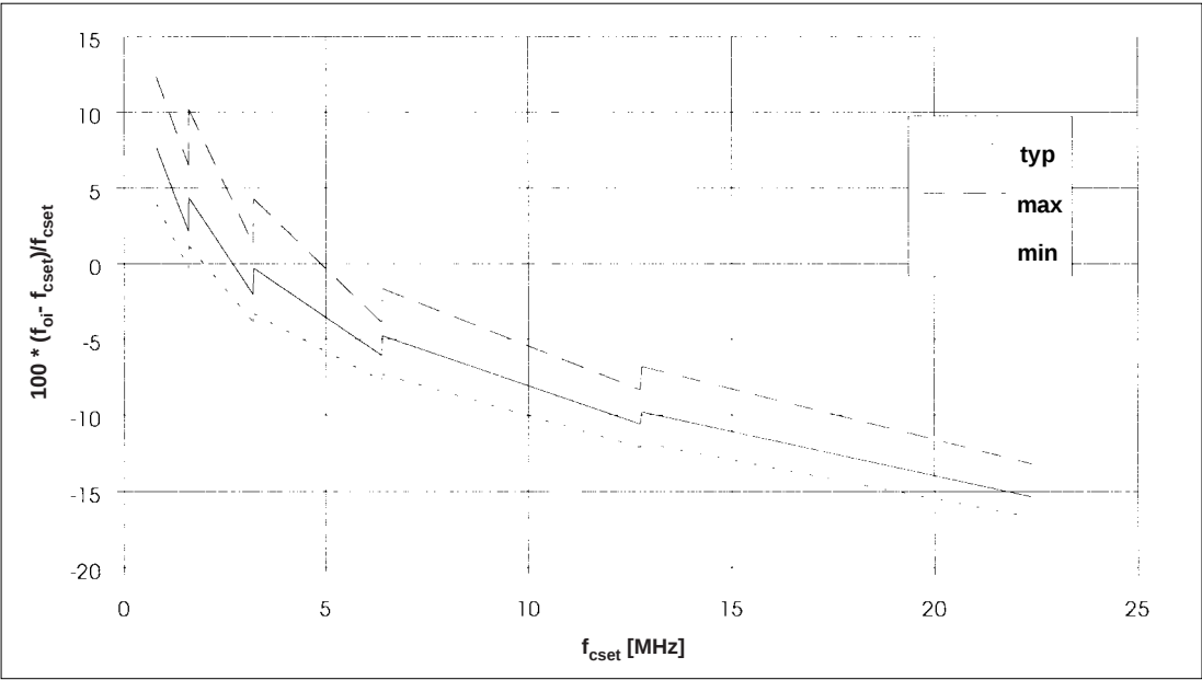
Figure 6: Measured oscillator frequency deviation vs. settings ( V_{EE} = -5.00 V / T_a = 25^\circ\text{C} )
