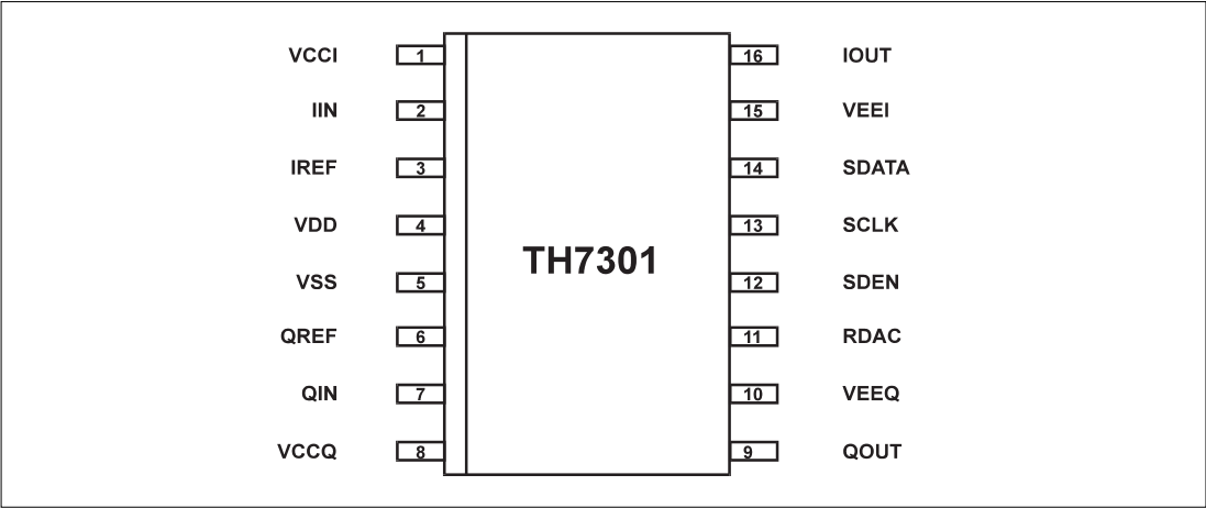
Figure 2: Pinout Schematic
