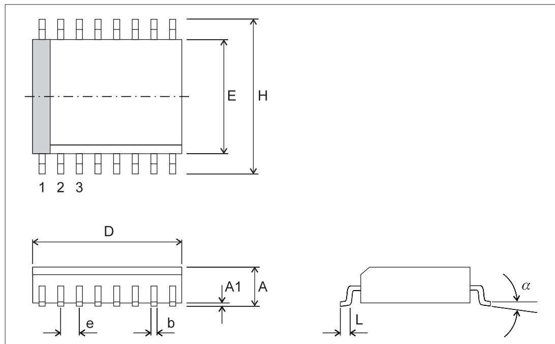
Small Outline Package (SOP) SOP 16 Wide Body (WB)
