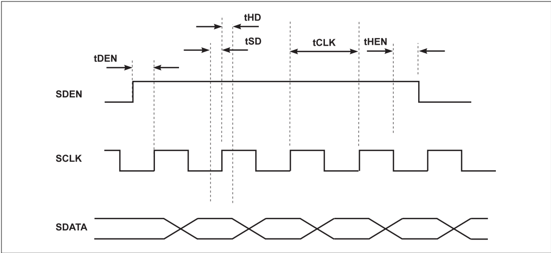
Figure 3: Serial Interface Timing Diagram
