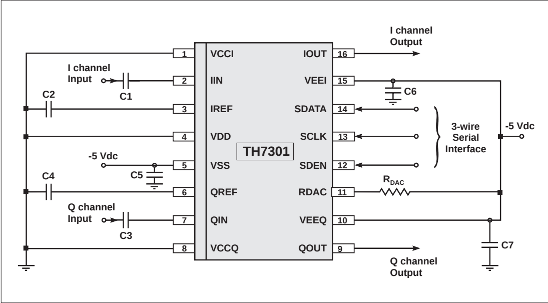
Figure 4: Application Diagram
