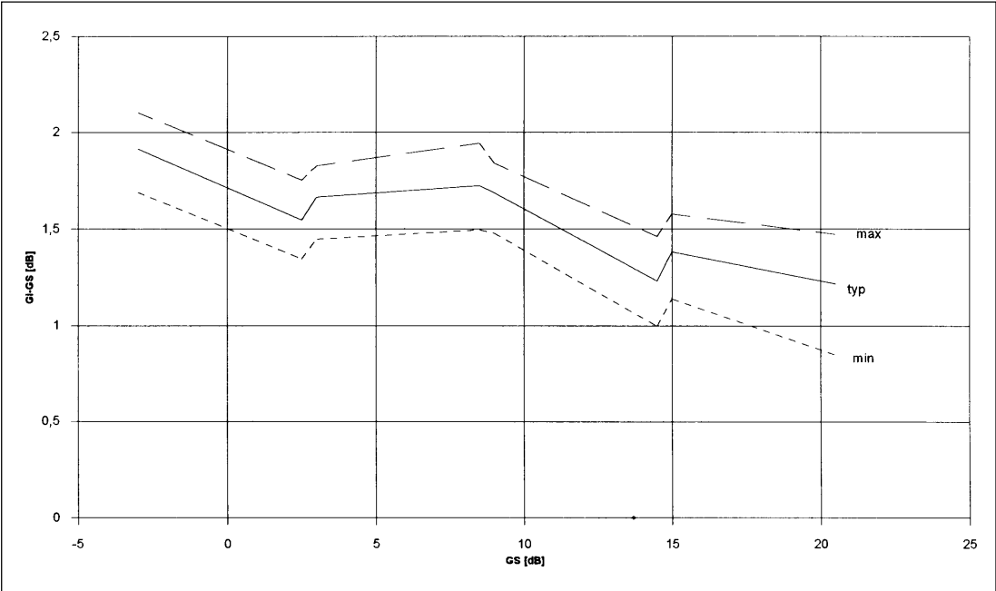
Figure 10: initial gain accuracy ( f_{cset} = 22.4 \text{ MHz} , f_{meas} = 5.0 \text{ MHz} , VEE = -5.0 \text{ V} , T_a = 23^\circ \text{ C} )
