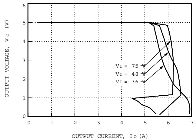
Figure 4. LW025A Typical Output Characteristics
