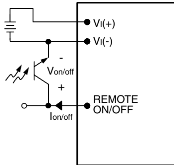
Figure 13. Remote On/Off Implementation
