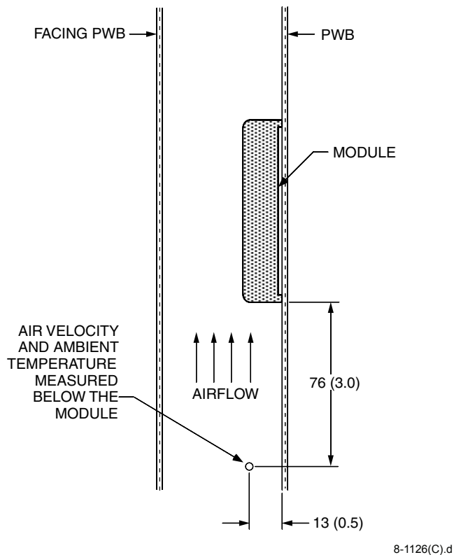
Figure 19. Experimental Test Setup
