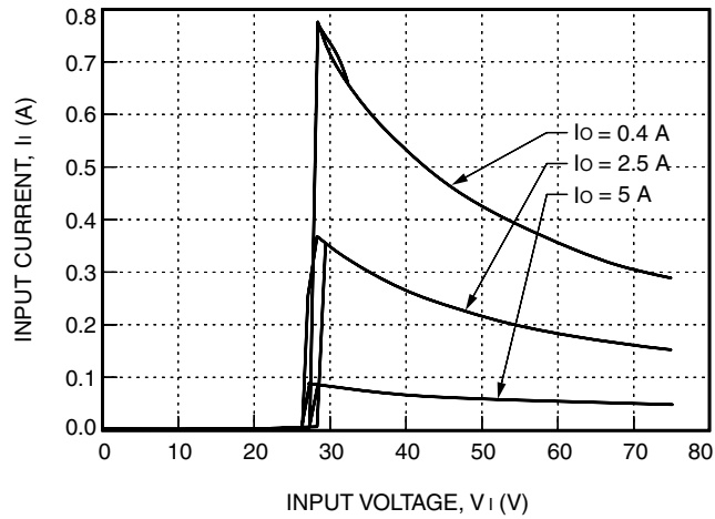
Figure 1. LW025F Typical Input Characteristics
