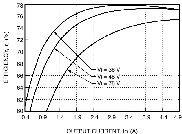
Figure 5. LW025F Typical Converter Efficiency vs. Output Current
