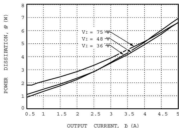
Figure 18. LW025A Power Dissipation vs. Output Current, T_a = 25^\circ\text{C}
