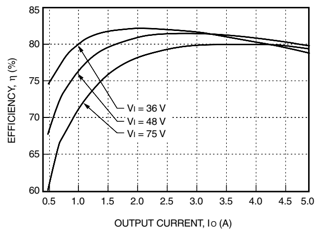
Figure 6. LW025A Typical Converter Efficiency vs. Output Current
