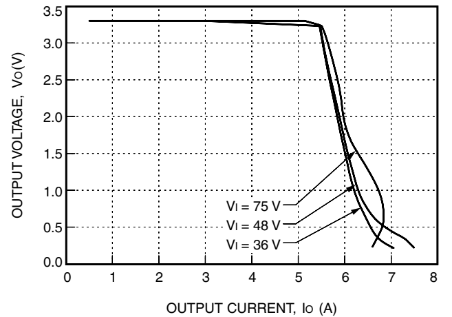
Figure 3. LW025F Typical Output Characteristics
