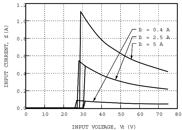
Figure 2. LW025A Typical Input Characteristics
