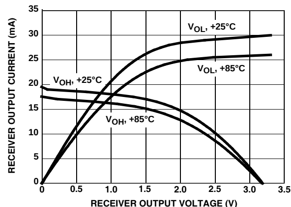
FIGURE 23. RECEIVER OUTPUT CURRENT vs RECEIVER OUTPUT VOLTAGE
