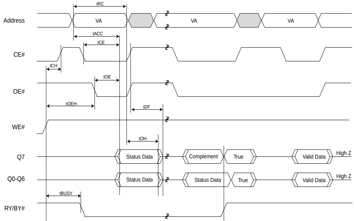
Figure 22. DATA# POLLING TIMING WAVEFORMS (DURING AUTOMATIC ALGORITHMS)
