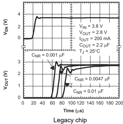
Figure 5-21. TPS793 Output Voltage, Enable Voltage vs Time (Start-Up)
