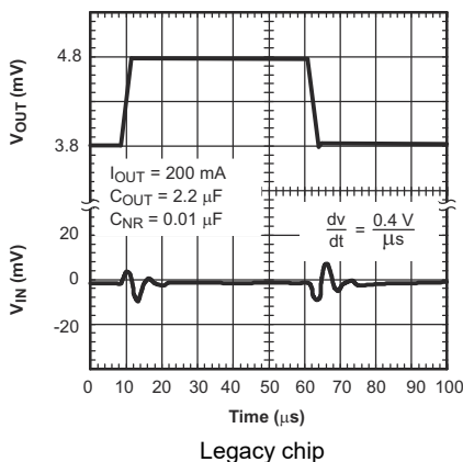
Figure 5-23. TPS793 Line Transient Response
