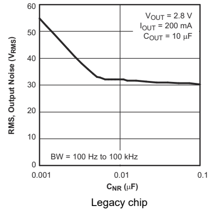
Figure 5-10. Root Mean Square Output Noise vs C_{NR}
