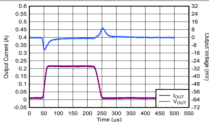
Figure 7-7. TPS79328 Load Transient Response
