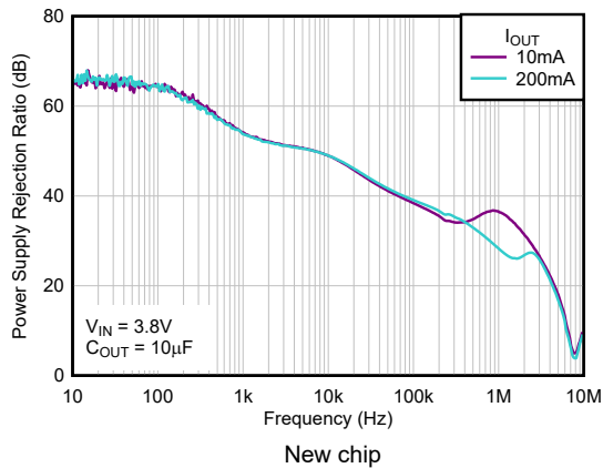
Figure 5-19. TPS793 Ripple Rejection vs Frequency
