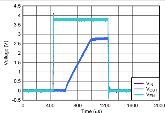
Figure 7-5. TPS79328 Output Voltage, Enable Voltage vs Time (Start-Up)
