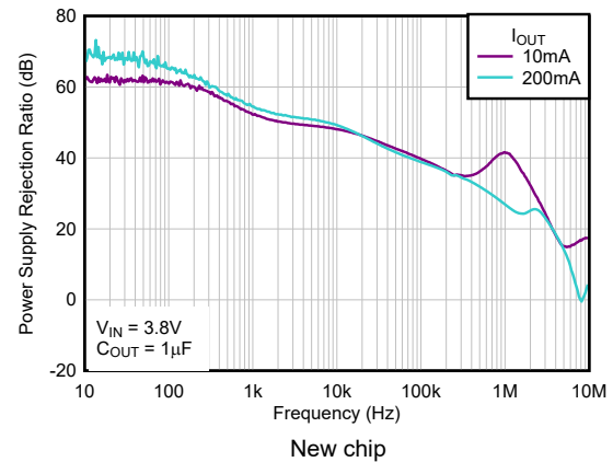
Figure 5-20. TPS793 Ripple Rejection vs Frequency
