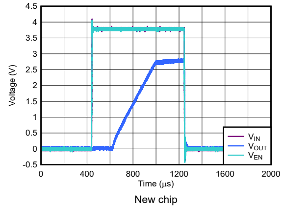
Figure 5-22. TPS793 Output Voltage, Enable Voltage vs Time (Start-Up)
