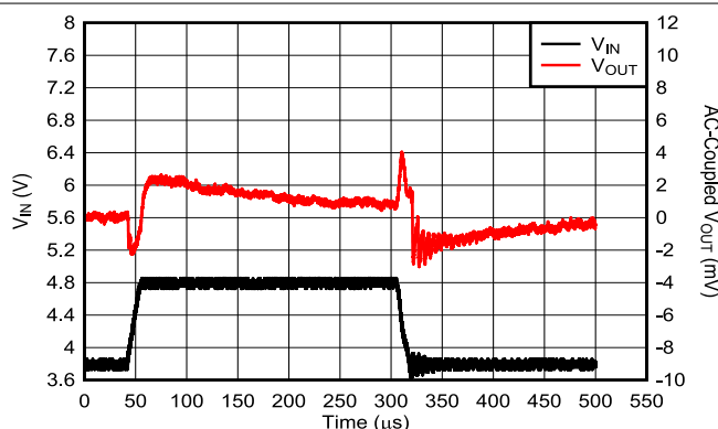
Figure 7-6. TPS79328 Line Transient Response
