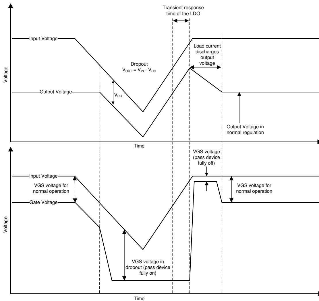
Figure 7-3. Line Transients From Dropout
