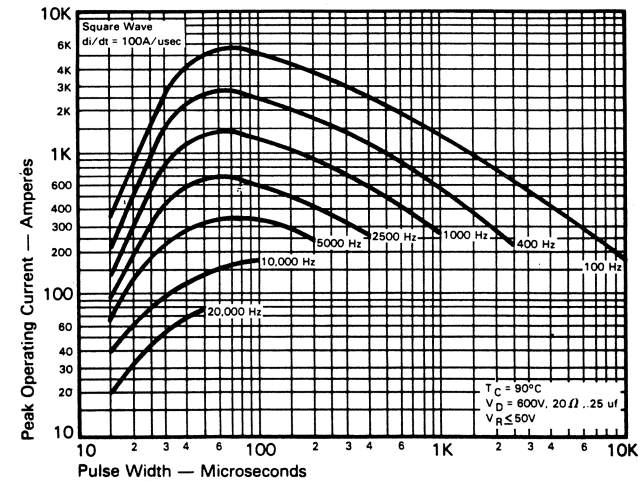
MAXIMUM ALLOWABLE PEAK ON-STATE CURRENT vs. PULSE WIDTH ( di/dt = 100\text{A}/\text{usec} )
