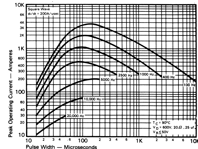
MAXIMUM ALLOWABLE PEAK ON-STATE CURRENT vs. PULSE WIDTH ( di/dt = 200\text{A}/\text{usec} )
