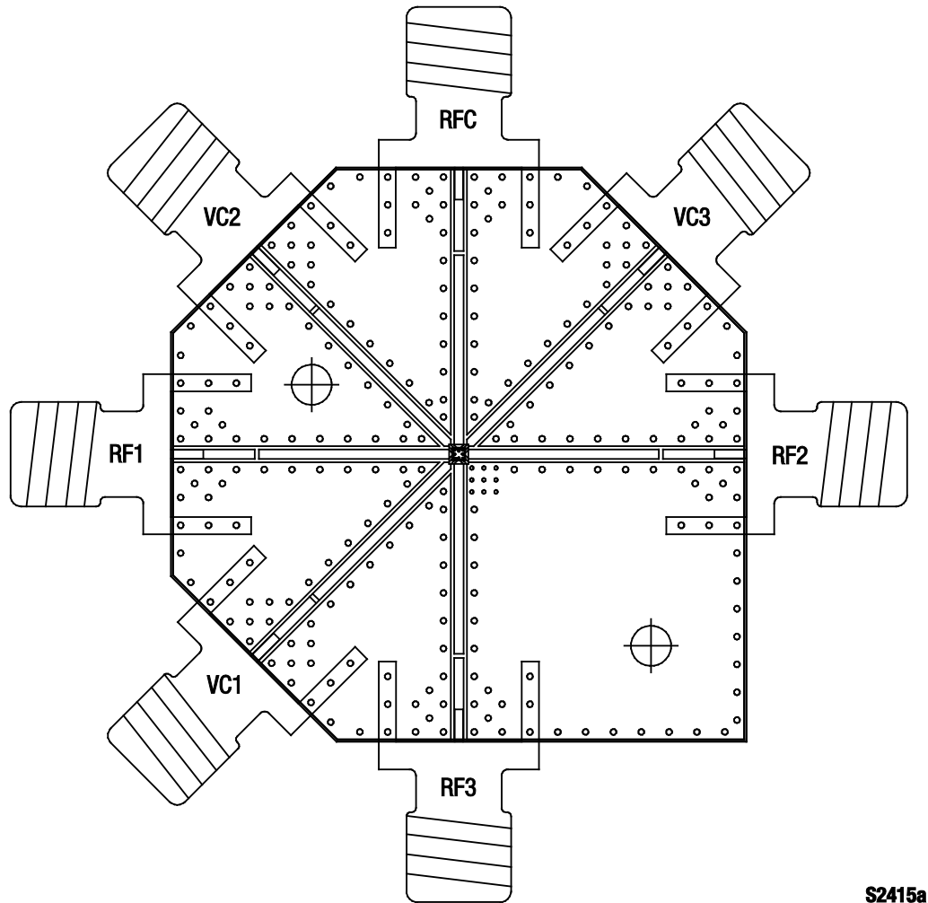
Figure 9. SKY13386-000 Evaluation Board Assembly Diagram
