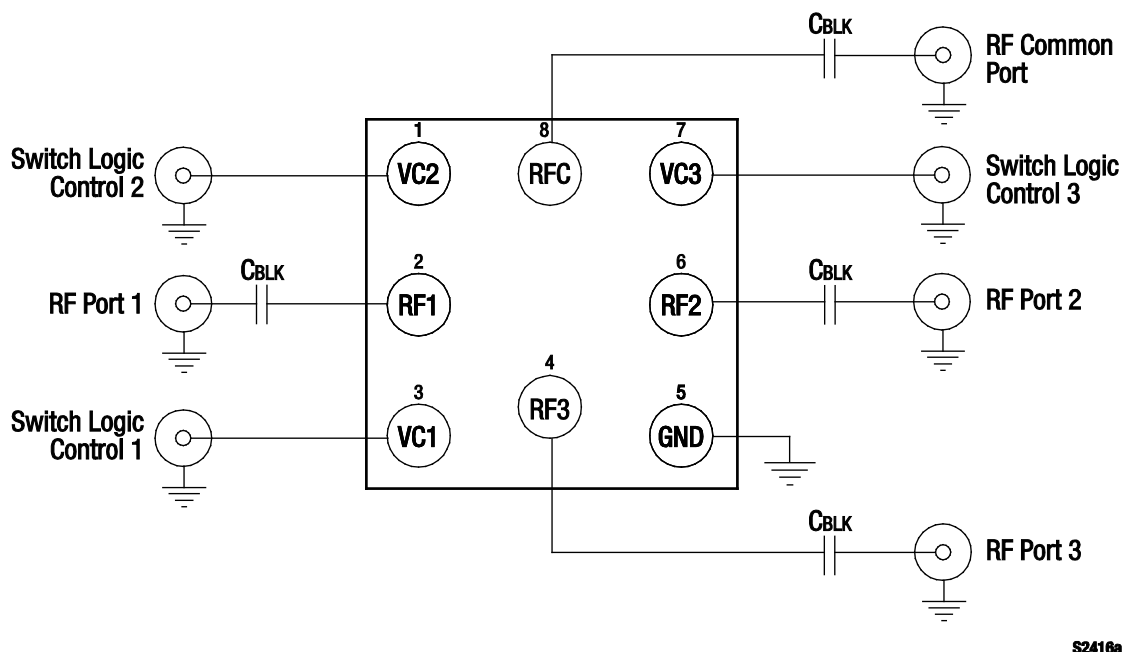
Figure 8. SKY13386-000 Evaluation Board Schematic
