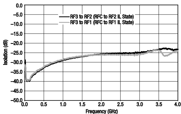
Figure 7. Port-to-Port Isolation vs Frequency
