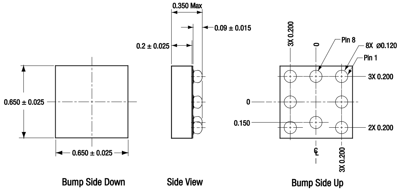
Figure 10. SKY13386-000 8-Bump CSP Package Dimensions
