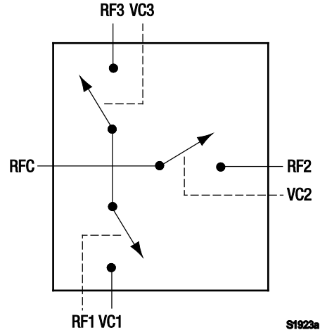
Figure 1. SKY13386-000 Block Diagram
