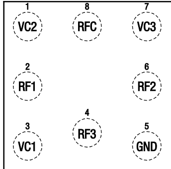
Figure 2. SKY13386-000 Pinout – 8-Bump CSP (Top View, Bumps Down)
