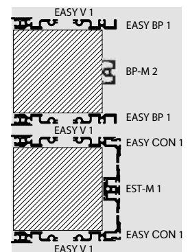
2 Top: for backplane Bottom: for connector
