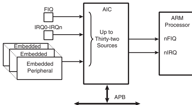
Figure 16-1. Block Diagram
