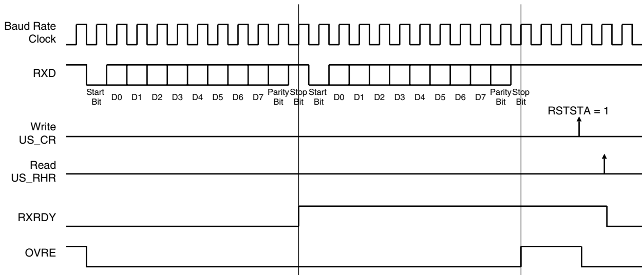
Figure 24-10. Receiver Status
