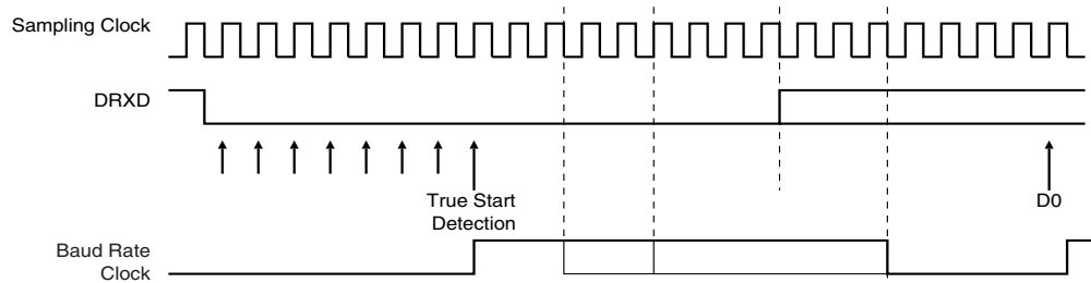
Figure 20-4. Start Bit Detection
