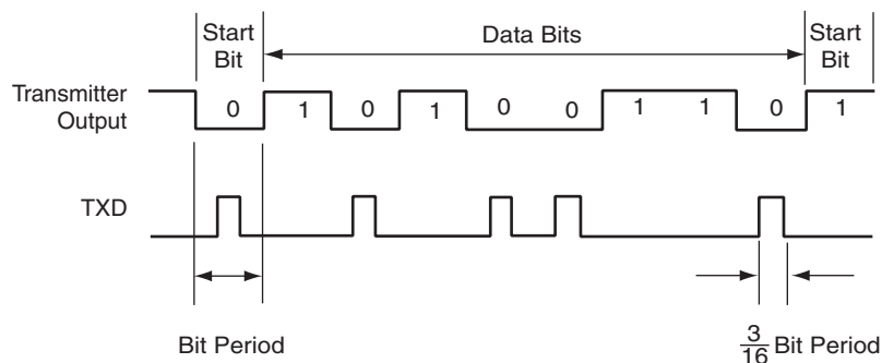
Figure 24-23. IrDA Modulation
