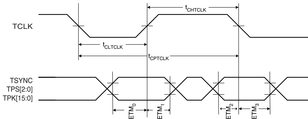
Figure 32-11. ETM Signals
