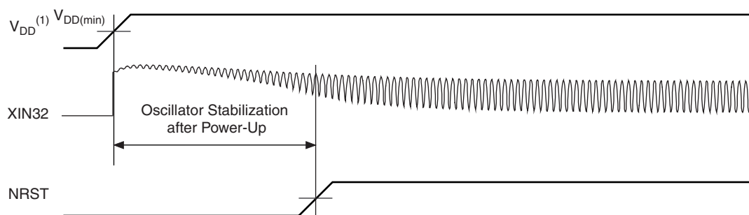
Figure 9-1. Cold Reset and Oscillator Start-up relationship
