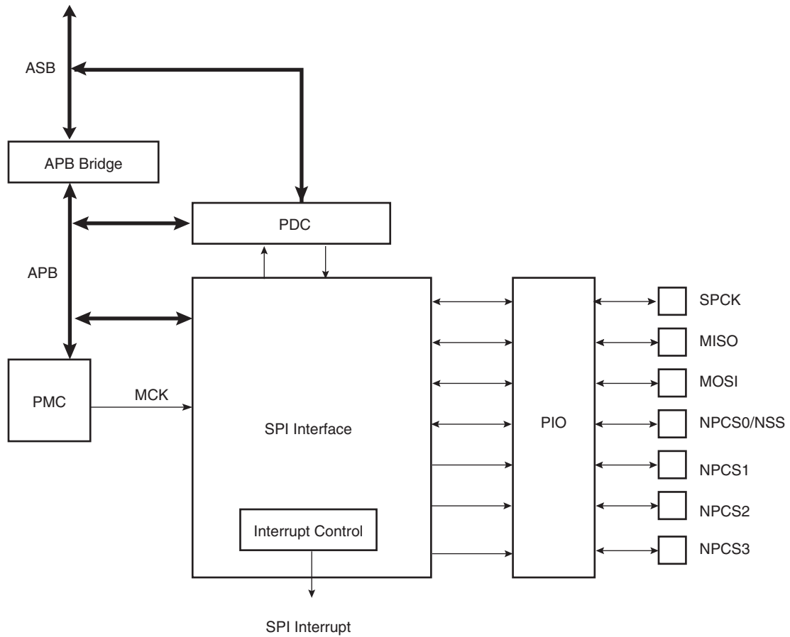
Figure 22-1. Block Diagram
