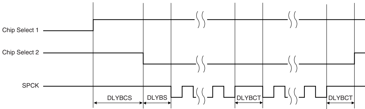
Figure 22-3. Programmable Delays
