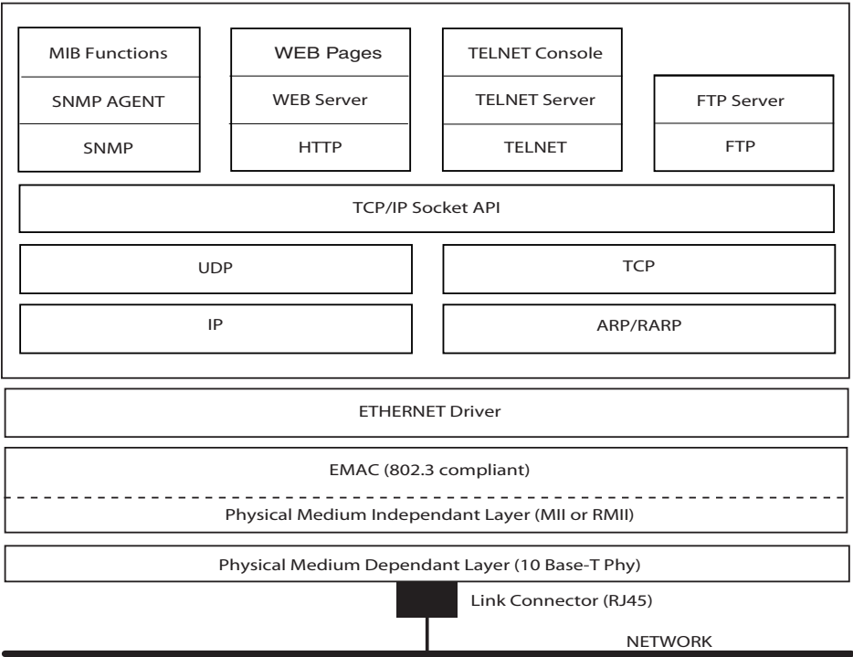
Figure 30-2. Ethernet MAC Application Block Diagram
