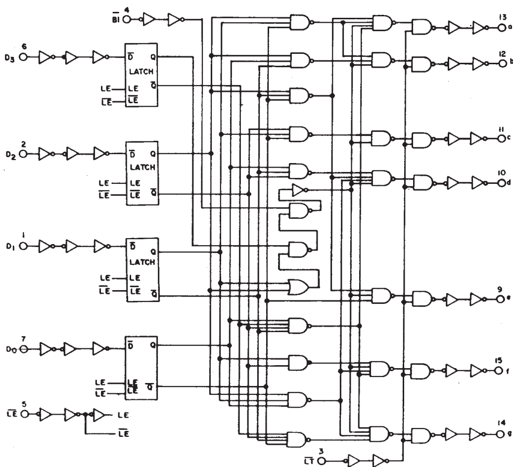
Fig. 1 - Logic diagram.
