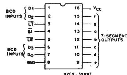
TERMINAL ASSIGNMENT
