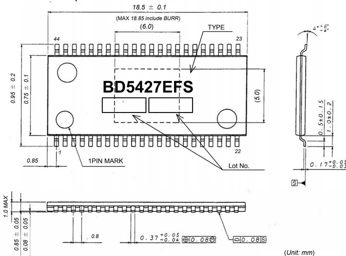
Fig. 23 Outer Dimensions and Inscriptions of HTSSOP-A44 Package
