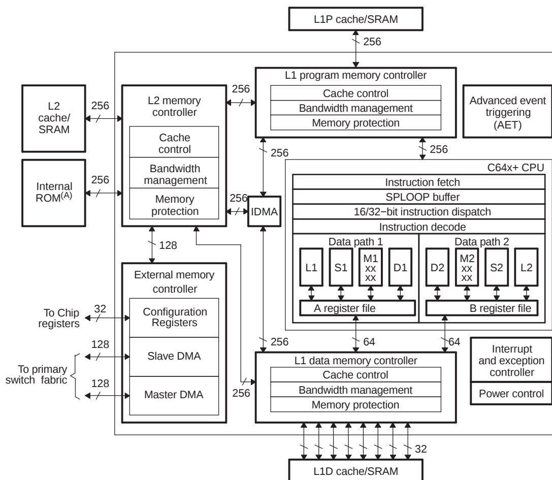
Figure 5-1. 64x+ Megamodule Block Diagram
