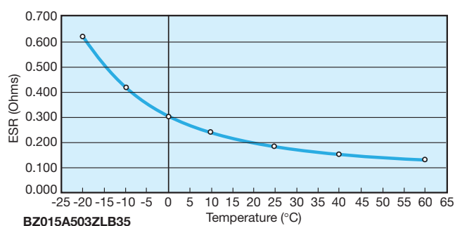
ESR Comparison
