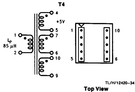
FIGURE 18. Collcraft Q4344-B
