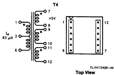
FIGURE 28. Renco RL-5535
