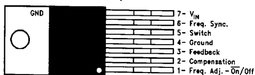
Bent, Staggered Leads 7-Lead TO-220 (T) Top View
