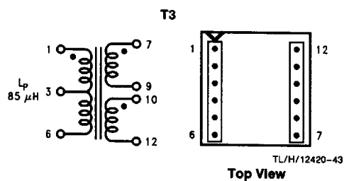
FIGURE 27. Renco RL-5534
