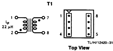
FIGURE 15. Collcraft Q4434-B
