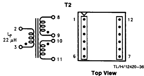
FIGURE 20. Collcraft Q4436-B (Surface Mount)
