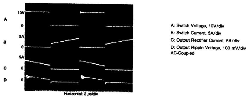
FIGURE 5. Switching Waveforms
