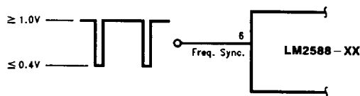
FIGURE 43. Frequency Synchronization
