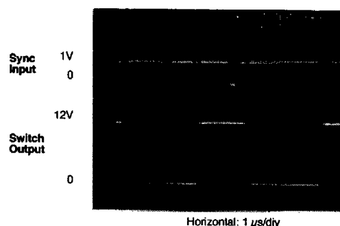
FIGURE 44. Waveforms of a Synchronized 12V Boost Regulator
