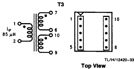
FIGURE 17. Collcraft Q4343-B
