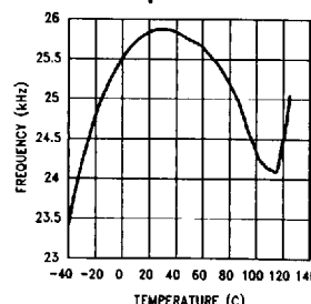
Short Circuit Frequency vs Temperature
