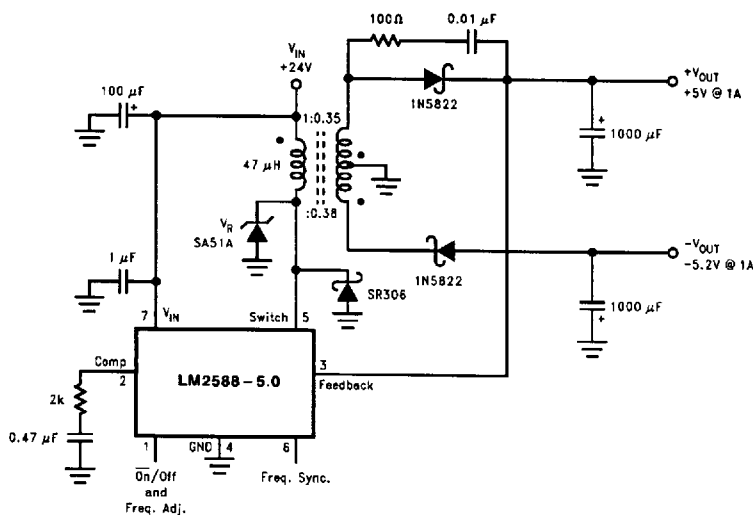
FIGURE 46. Flyback Regulator
