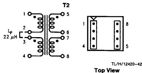
FIGURE 26. Renco RL-5531
