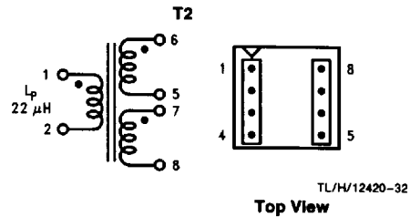
FIGURE 16. Collcraft Q4337-B
