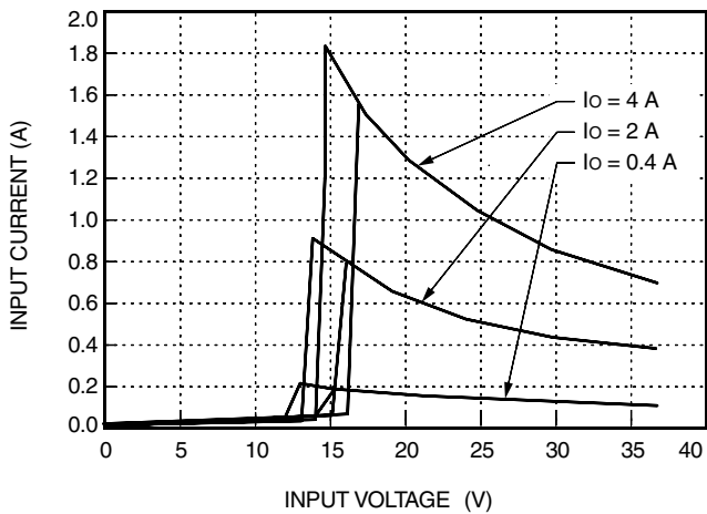
Figure 2. LC020A Typical Input Characteristics, T_A = 25\text{ }^{\circ}\text{C}
