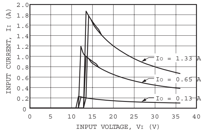
Figure 4. LC020C Typical Input Characteristics, T_A = 25\text{ }^{\circ}\text{C}
