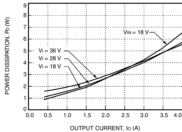
Figure 23. LC020A Power Dissipation vs. Output Current, T_A = 25\text{ }^\circ\text{C}
