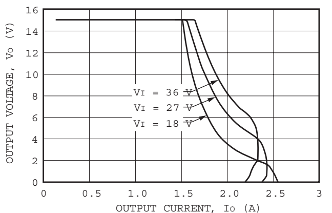
Figure 8. LC020C Typical Output Characteristics, T_A = 25^\circ\text{C}
