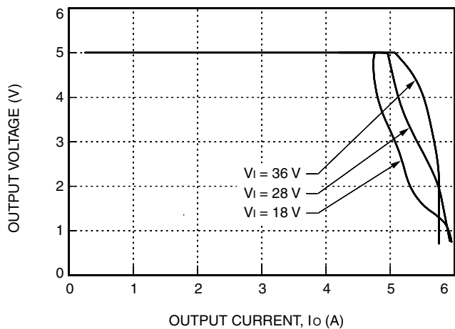
Figure 6. LC020A Typical Output Characteristics, T_A = 25^\circ\text{C}
