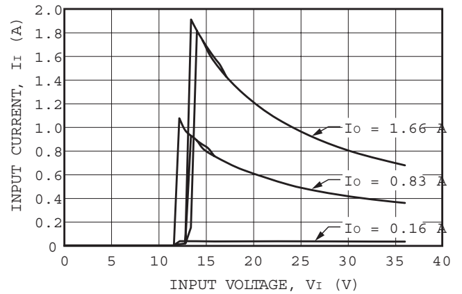
Figure 3. LC020B Typical Input Characteristics, T_A = 25\text{ }^{\circ}\text{C}
