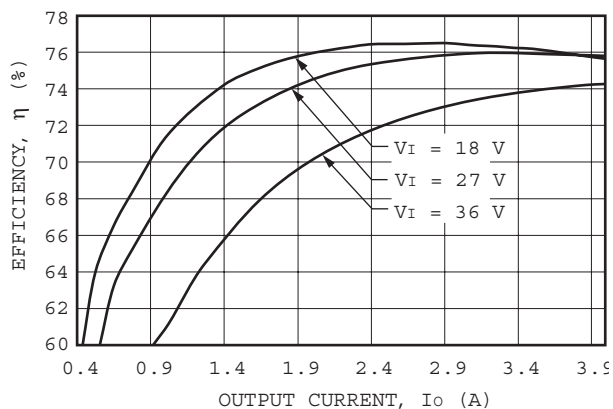
Figure 9. LC020F Typical Converter Efficiency vs. Output Current, T_A = 25 °C
