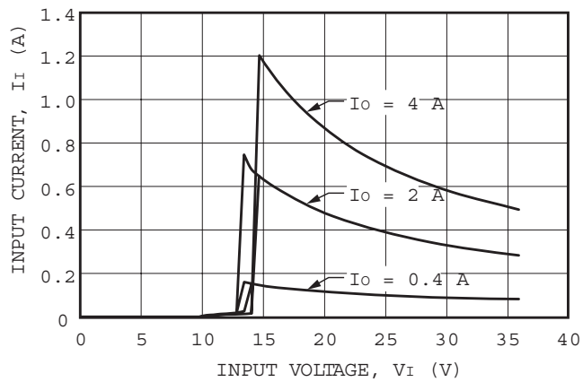
Figure 1. LC020F Typical Input Characteristics, T_A = 25\text{ }^{\circ}\text{C}
