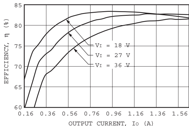
Figure 11. LC020B Typical Converter Efficiency vs. Output Current, T_A = 25 °C
