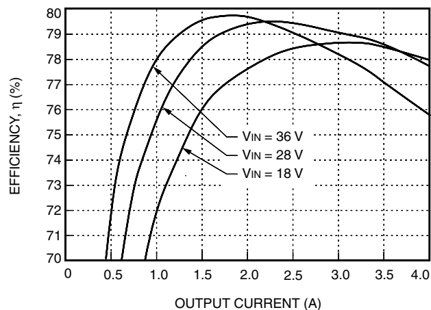
Figure 10. LC020A Typical Converter Efficiency vs. Output Current, T_A = 25 °C
