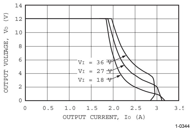
Figure 7. LC020B Typical Output Characteristics, T_A = 25^\circ\text{C}
