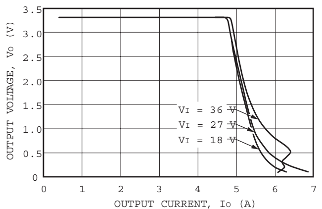
Figure 5. LC020F Typical Output Characteristics, T_A = 25^\circ\text{C}
