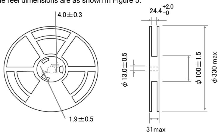
Figure 5 Reel Forms
