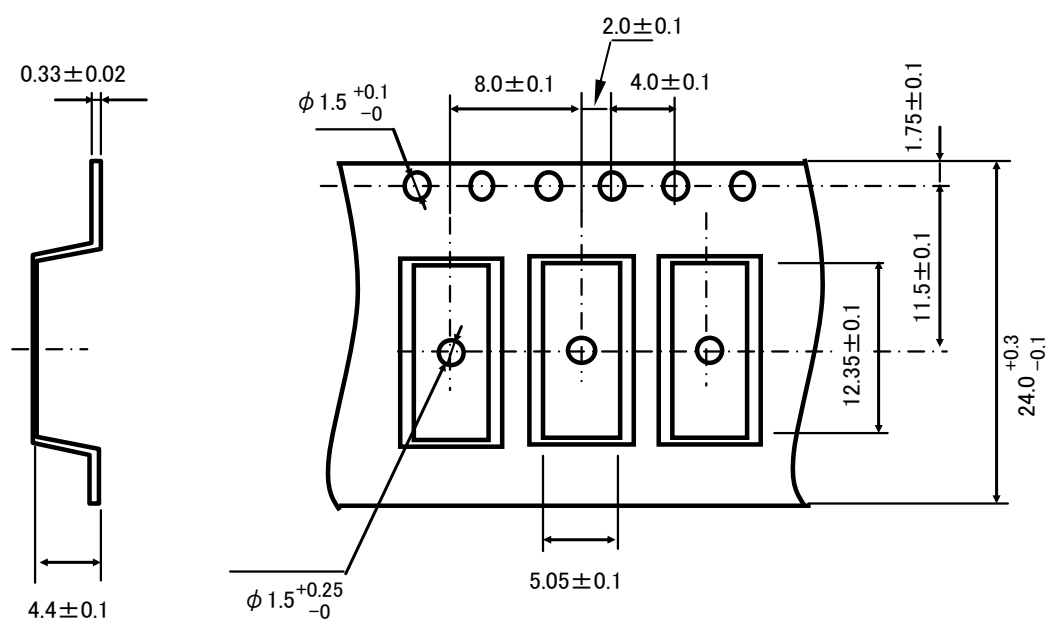
Figure 3 Tape Forms
