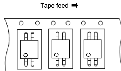
Figure1 Device Orientation
