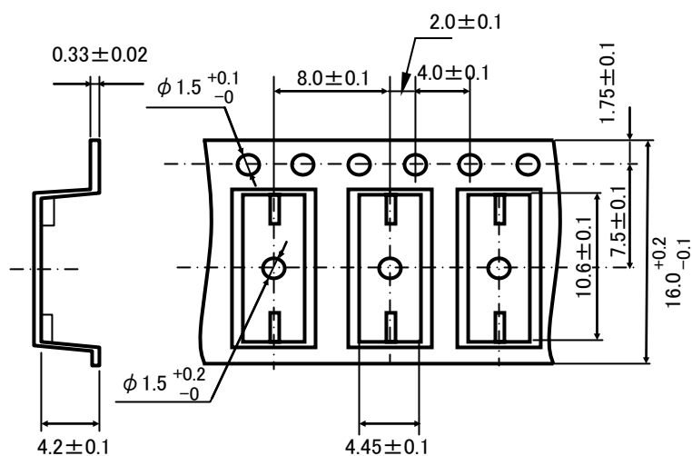
Figure 2 Tape Forms
