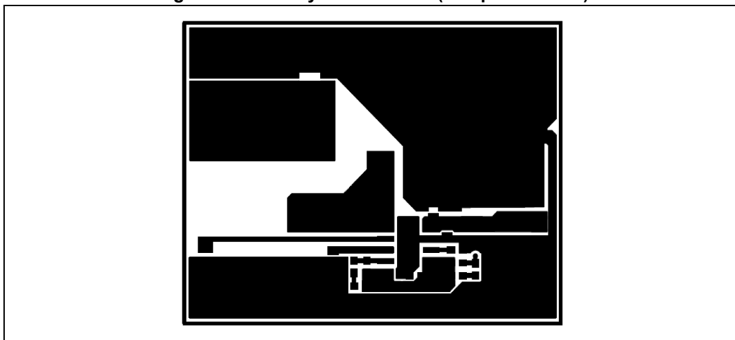
Figure 19. PCB layout: L7986TA (bottom side)
