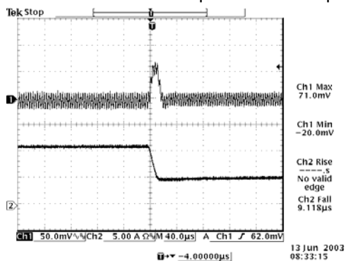
100% to 50% load 3.3 Vdc Input 1.5 Vdc Output
