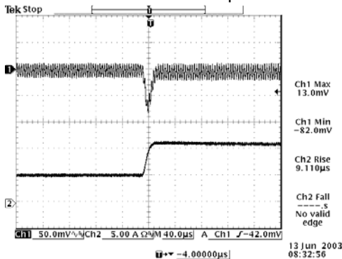
50% to 100% load 3.3 Vdc Input 1.5 Vdc Output
