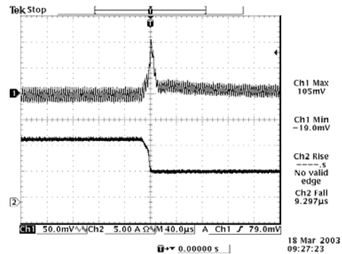
100% to 50% load 3.3 Vdc Input 1.8 Vdc Output
