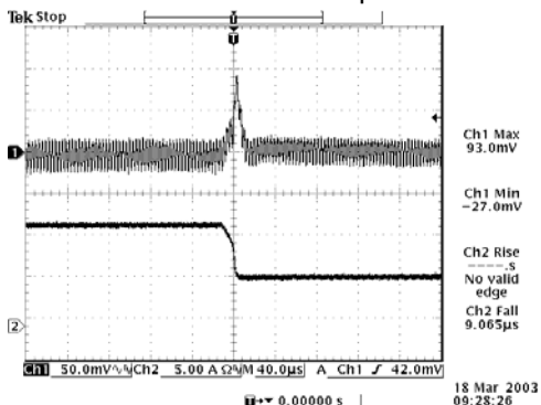
100% to 50% load 5 Vdc Input 1.8 Vdc Output
