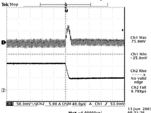
100% to 50% load 5 Vdc Input 1.5 Vdc Output
