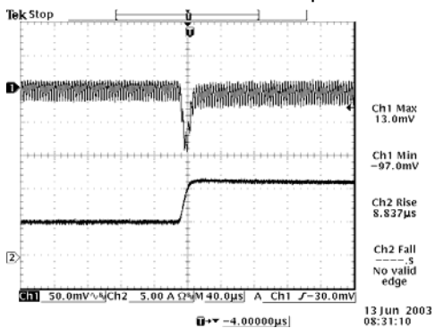
50% to 100% load 5 Vdc Input 1.5 Vdc Output
