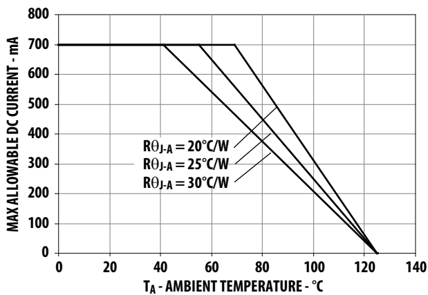
Figure 8. Maximum Forward Current vs. Ambient Temperature. Derated based on T_{JMAX} = 125^{\circ}\text{C} , R_{\theta JA} = 20^{\circ}\text{C/W} , 25^{\circ}\text{C/W} and 30^{\circ}\text{C/W} .
