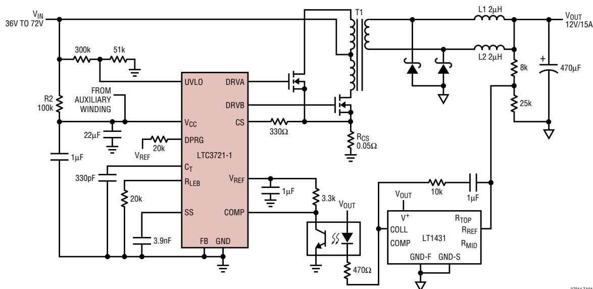
Isolated 36V to 72V DC to 12V/15A Push-Pull Converter
