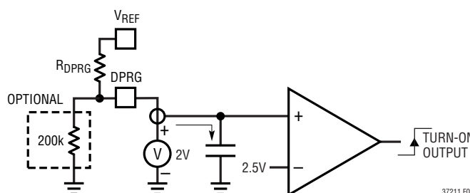
Figure 1. Deadtime Adjust
