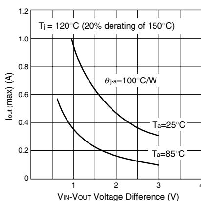
Allowable Output Current (vs. V_{IN}-V_{OUT} Voltage Difference) V_{IN}-I_O \text{ max}
