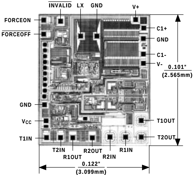
Chip Topography
