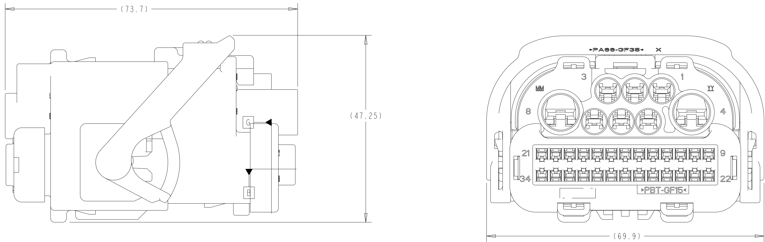
MATED ASSEMBLY SCALE 2:1
