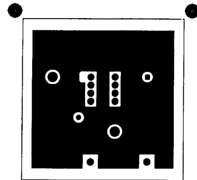
TOP LAYOUT
