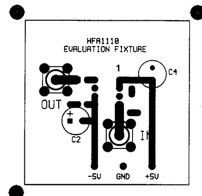
TOP LAYOUT
