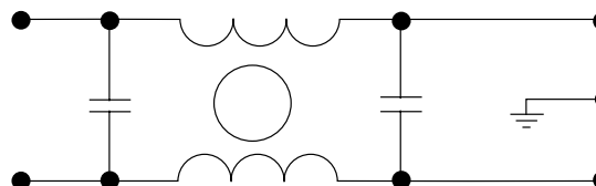
Circuit 2
