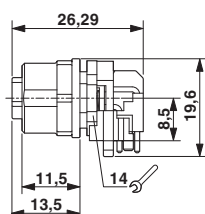
Dimensional drawing
